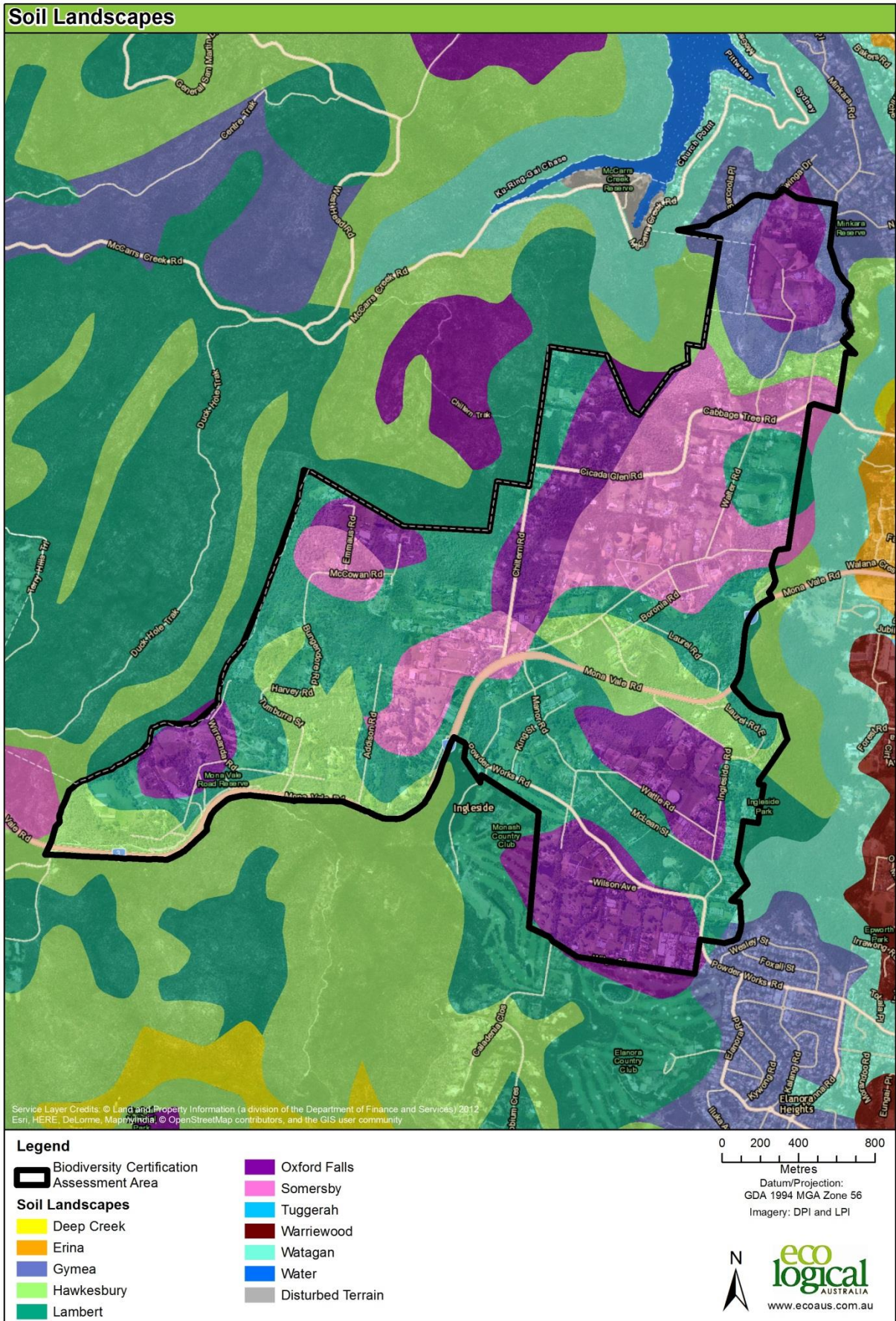
Figure 3: Soil landscape
